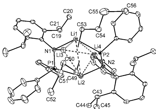
Figure 1. Crystal structure of [(\text{DipNPPPh})_2\text{Li}_4n\text{Bu}_2] ( 2 ). The thermal ellipsoids are shown at 30% probability. Hydrogen atoms have been omitted for clarity. Only the main components of the disordered n -butyl groups are shown. Selected bond lengths [Å] and angles [°]: P1–N1 1.6786(13), P2–N2 1.6785(13), Li1–N1 2.034(3), Li1–P2 2.560(3), Li2–N2 2.072(3), Li2–P1 2.591(3), Li3–N1 2.023(2), Li3–P1 2.962(3), Li4–N2 2.018(3), Li4–P2 2.884(3), Li2–C49 2.256(3), Li3–C49 2.218(3), Li4–C49 2.202(3), Li1–C53 2.270(3), Li3–C53 2.217(3), Li4–C53 2.245(3), Li1–Li2 3.218(4), Li1–Li3 2.407(4), Li1–Li4 2.856(4); N1–P1–Li2 94.89(7), P1–N1–Li1 112.26(10), P1–N1–Li3 105.92(10), Li3–Li1–Li4 57.04(10), Li3–Li1–Li2 58.67(10), Li4–Li1–Li2 46.57(8), Li4–Li2–Li3 57.07(10), Li4–Li2–Li1 58.84(10), Li3–Li2–Li1 46.29(8), Li1–Li3–Li4 70.40(12), Li1–Li3–Li2 75.04(11), Li4–Li3–Li2 53.11(10), Li2–Li4–Li1 74.58(11), Li3–Li4–Li1 52.56(10).
