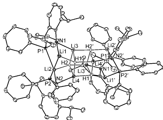
Figure 2. Crystal structure of [(\text{DipNPPPh})_2\text{Li}_4(\text{LiH})_4]\cdot\text{C}_6\text{H}_6 ( 3 · \text{C}_6\text{H}_6 ). The thermal ellipsoids are shown at 30% probability. The solvent molecule and hydrogen atoms except hydride ligands have been omitted for clarity. Selected bond lengths [Å] and angles [°]: P1–N1 1.666(2), P2–N2 1.673(2), P1–Li2 2.530(4), N1–Li3 2.037(4), N1–Li1 2.042(4), Li1–P2 2.530(4), N2–Li4 2.032(4), N2–Li2 2.038(4), Li1–H1 1.83(4), Li2–H2 1.81(4), Li3–H2 1.98(4), Li3–H1 1.96(4), Li4–H1 1.99(4), Li4–H2 1.97(4), Li1–Li2 3.131(6), Li1–Li3 2.509(5), Li1–Li4 3.051(6), Li2–Li3 3.061(6), Li3–Li4 2.668(8), Li3–Li4 2.821(6), Li3–Li4 2.691(5), Li4–Li4' 2.682(8); H2–Li4–H1 88.3(18), Li3–H2–Li4 ca. 91.0, Li4–H1–Li4' ca. 87.8, Li4–H1'–Li3' ca. 89.2. Symmetry operation: #1 -x, y, -z + \frac{1}{2} ; #2 -x, -y + 1, -z .
